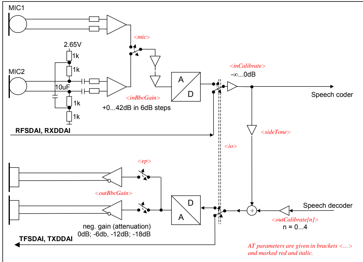
Figure 42: Audio programming model
